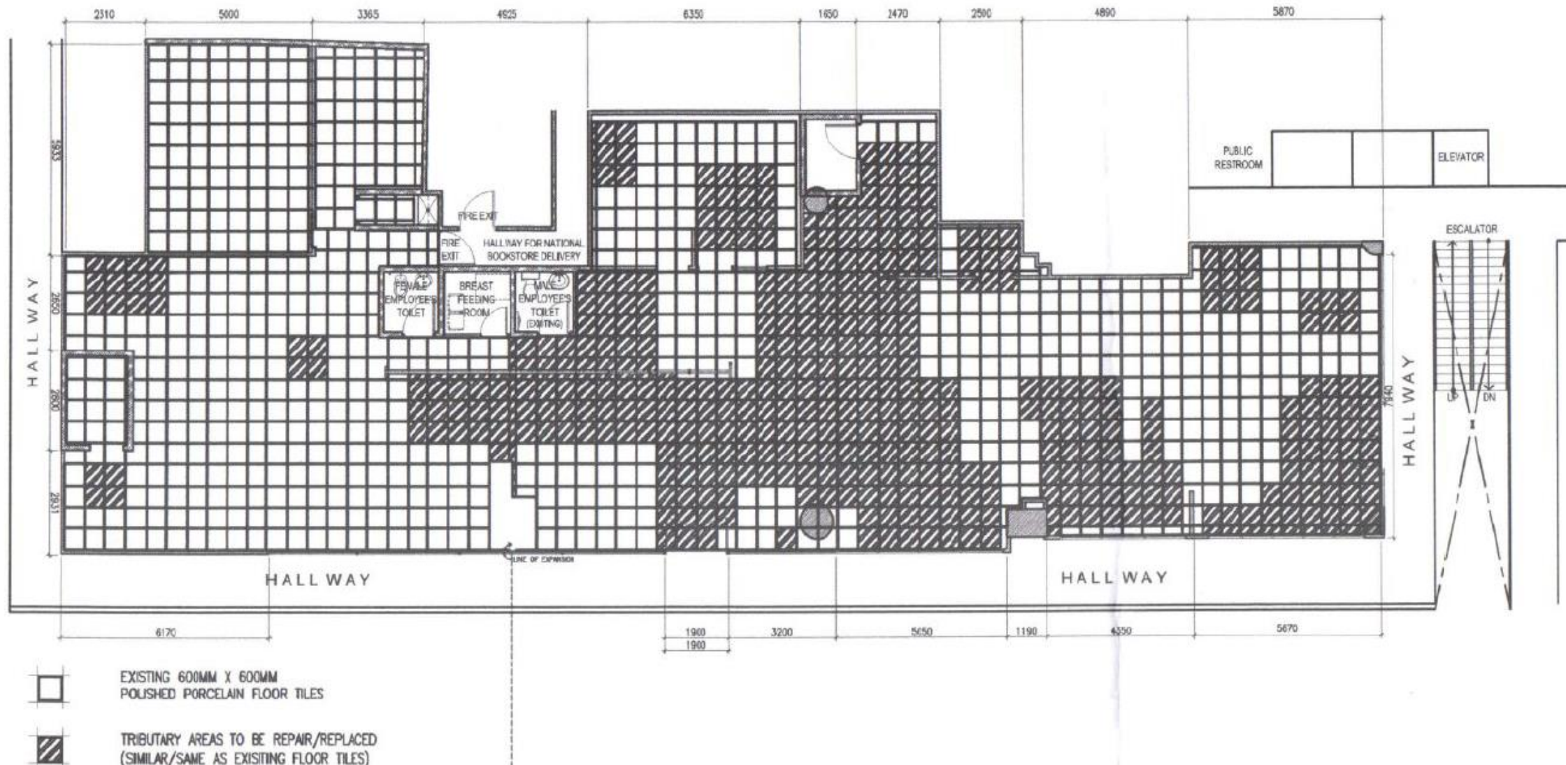
1 AREAS FOR REPAIR/REPLACEMENT OF POLISHED PORCELAIN FLOOR TILES A-1 SCALE 1:125 MTS.
