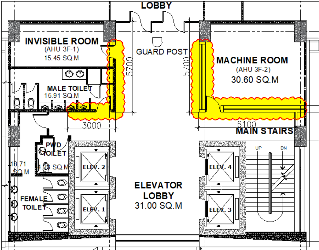
3 RD FLOOR TO 5 TH TYPICAL FLOOR PLAN
