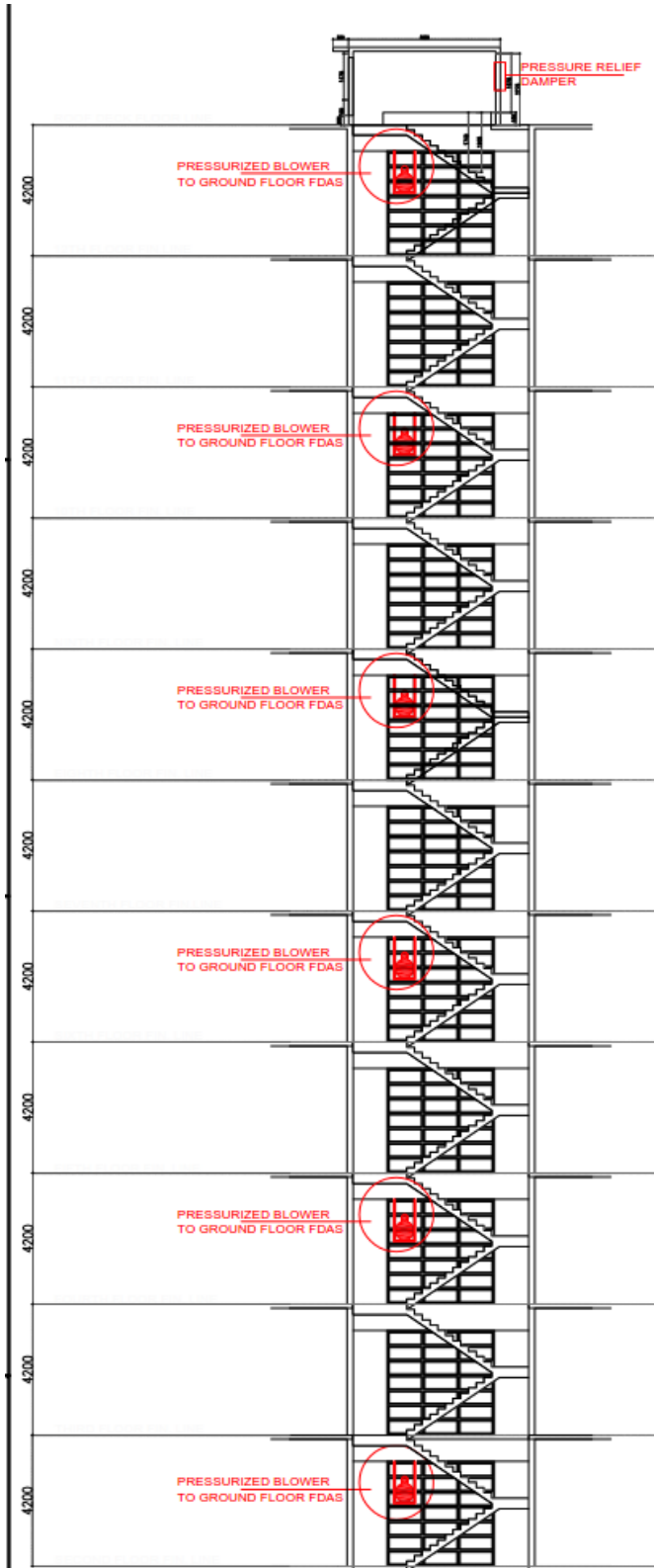
SECTION CUT GRID 14-15 SUPPRESSION DETAIL 3 S-01 SCALE 1:40
