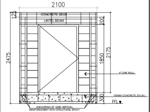
4 FRONT ELEVATION DETAIL S-01 SCALE 1:40
