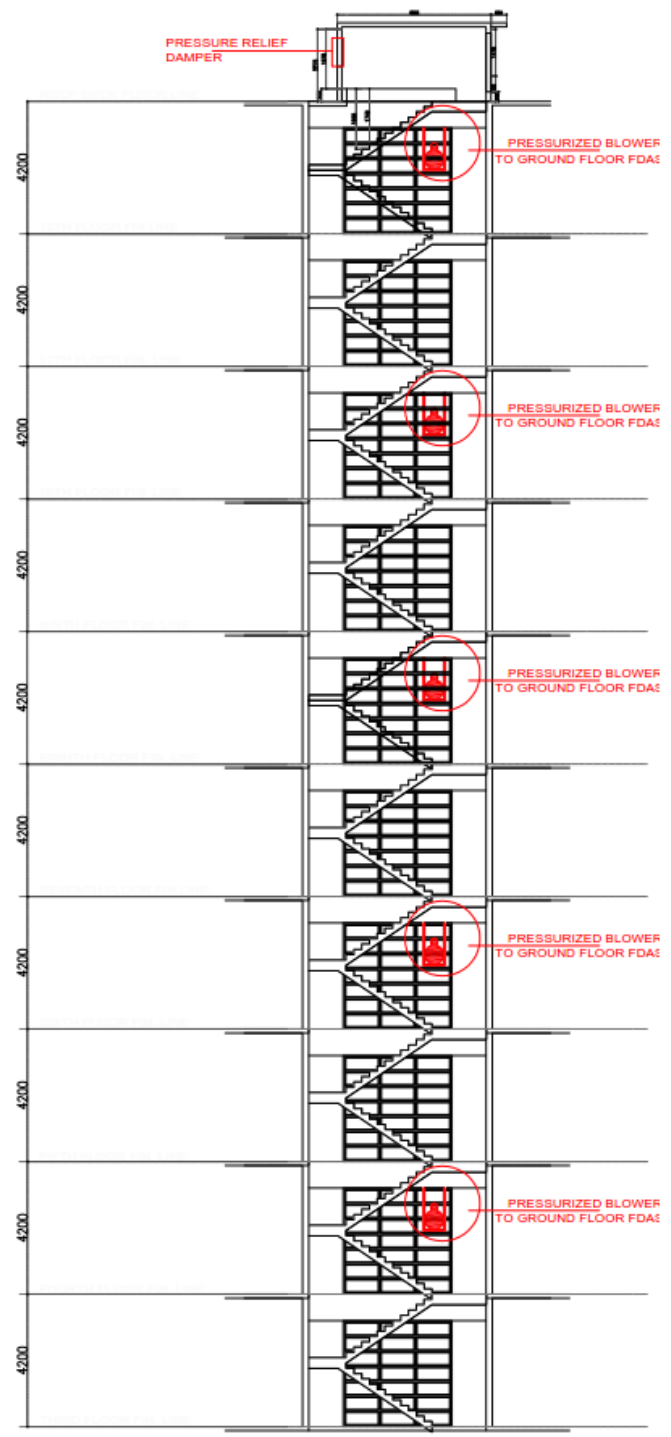
SECTION CUT GRID 1-2 SUPPRESSION DETAIL 3 S-01 SCALE 1:40
