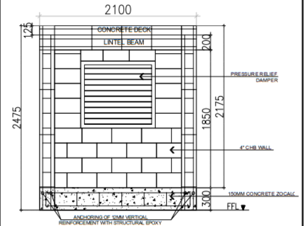
5 REAR ELEVATION DETAIL S-01 SCALE 1:40
