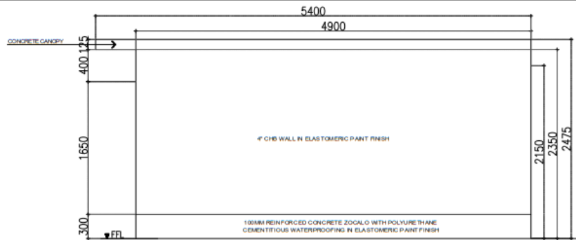
5 RIGHT SIDE ELEVATION DETAIL A-01 SCALE 1:40
