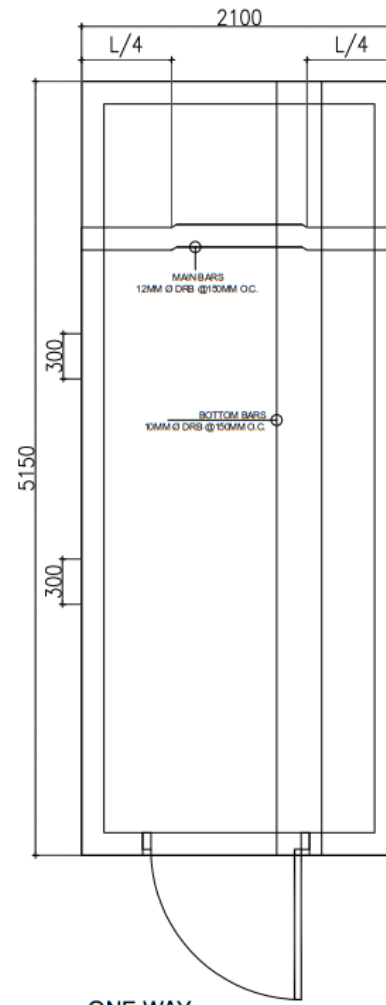
1 ONE WAY ROOF SLAB LAYOUT S-01 SCALE 1:40
