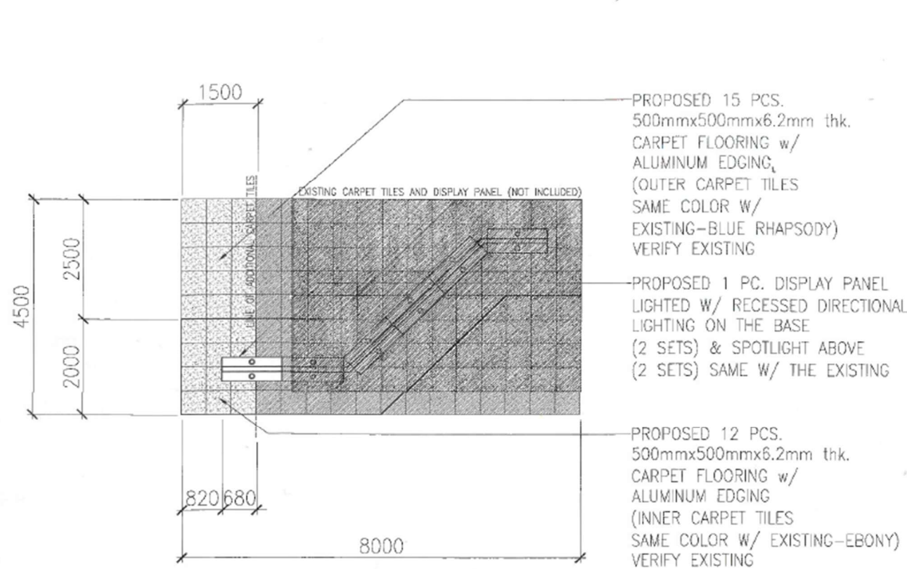
G/F MAIN LOBBY EXHIBIT DISPLAY AREA PROPOSED FLOOR LAYOUT
