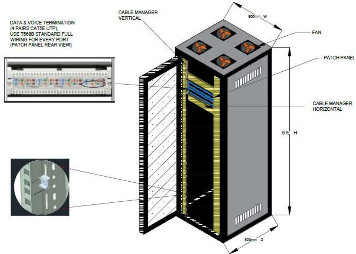
NETWORK DATA CABINET
