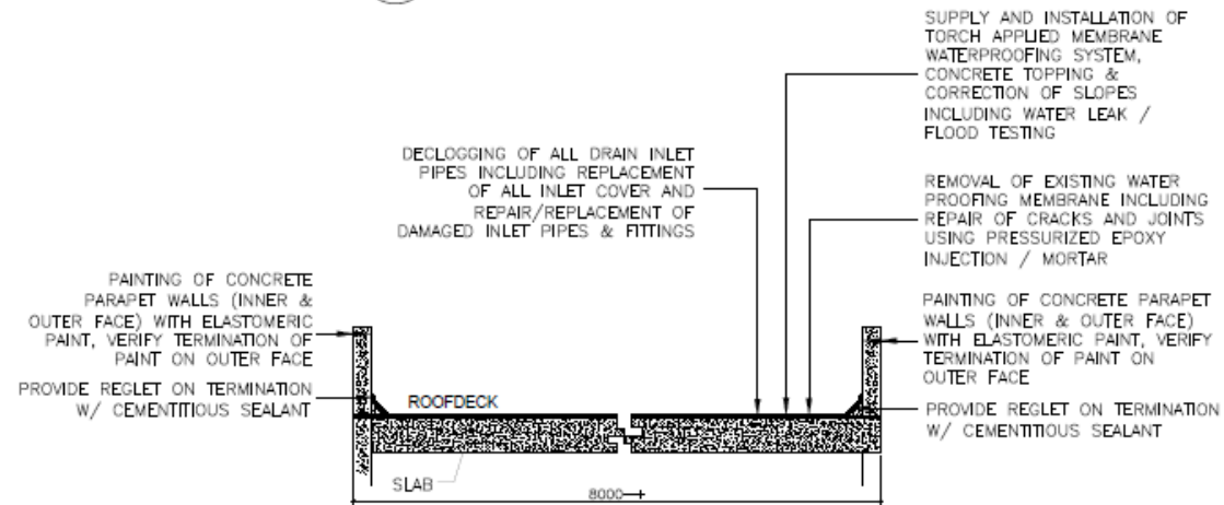
2 A-02 SCALE 1:50 M TYPICAL SECTION CONCRETE DECK
