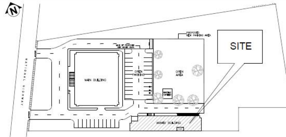
1 SITE DEVELOPMENT PLAN A-01 SCALE NTS
