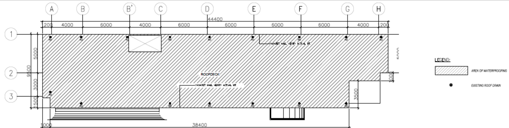
1 A-02 SCALE 1:200 M ANNEX BUILDING CONCRETE DECK PLAN
