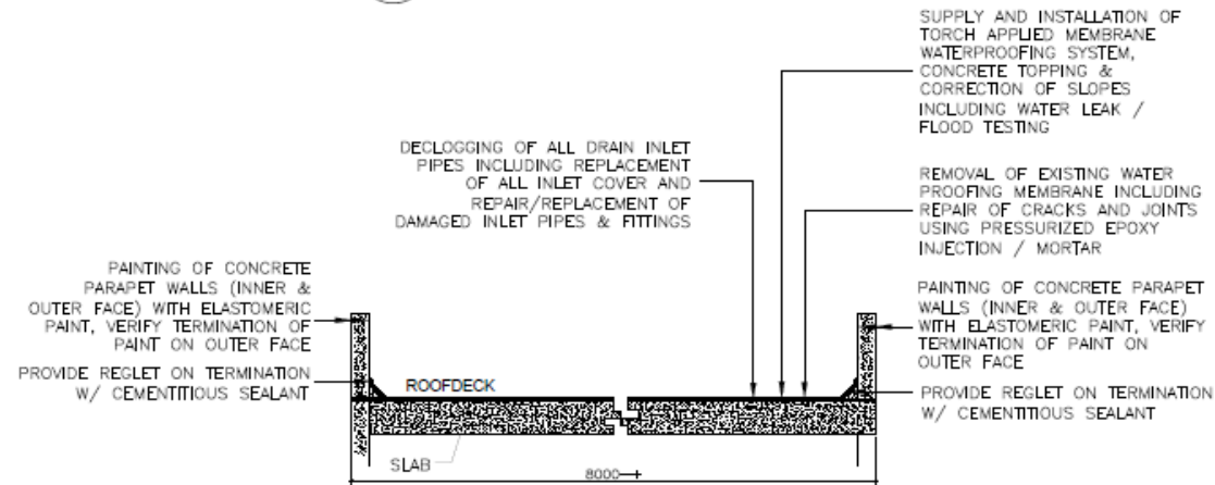
TYPICAL SECTION CONCRETE DECK 2 A-02 SCALE 1:50 M
