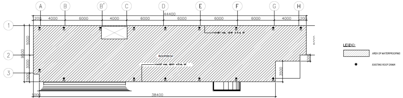
ANNEX BUILDING CONCRETE DECK PLAN 1 A-02 SCALE 1:200 M
