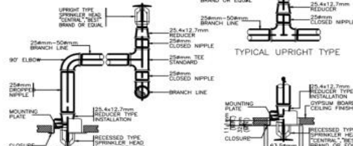
TYPICAL COMBINATION TYPE
