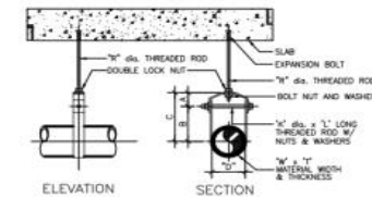
ELEVATION SECTION CLEVIS HANGERS
