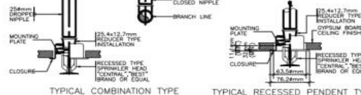
1 FP-01 DETAIL OF SPRINKLER HEADS
