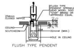
FLUSH TYPE PENDENT
