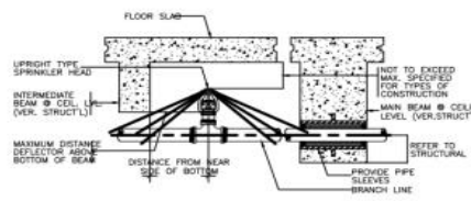
POSITION OF DEFLECTOR WHEN LOCATED ABOVE BOTTOM OF BEAM
