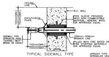
TYPICAL SIDEWALL TYPE
