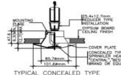
TYPICAL CONCEALED TYPE
