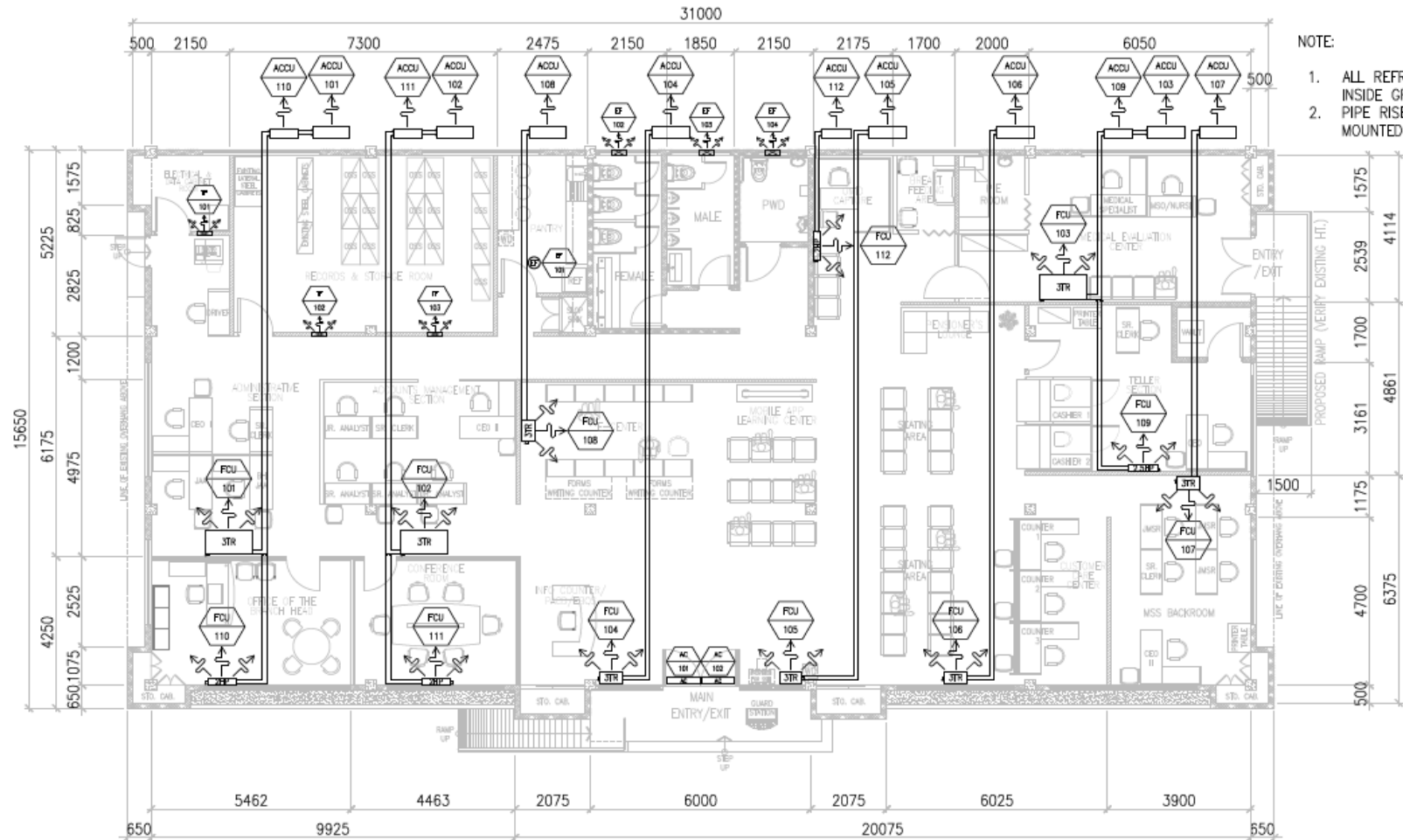
GROUND FLOOR PROPOSED MECHANICAL LAYOUT 1 M-03 SCALE 1:125
