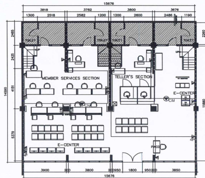
PROPOSED 1 1ST FLOOR LAYOUT
