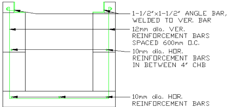
REINFORCEMENT DETAILS
