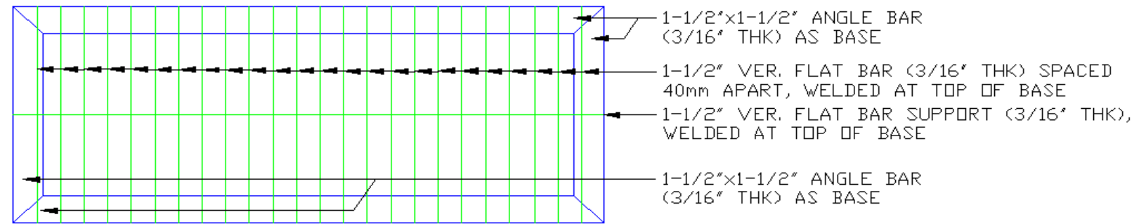
SEWER GRATE DETAILS
