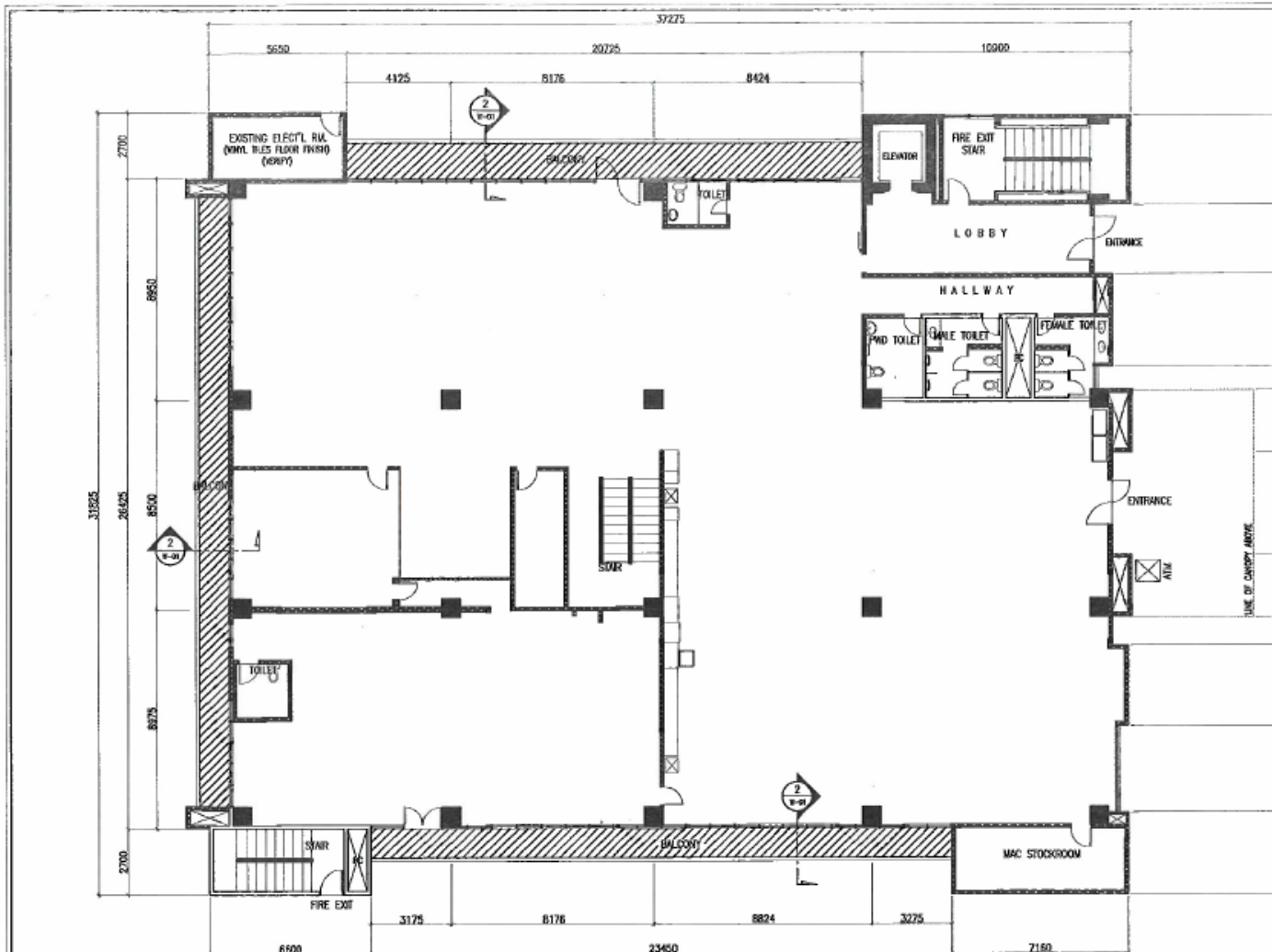
1 W-01 TYPICAL FLOOR PLAN 2nd - 4th FLOOR BALCONY SCALE 1:200
