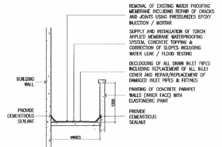
2 W-01 TYPICAL SECTION 2nd - 4th FLOOR BALCONY SCALE 1:50 M
