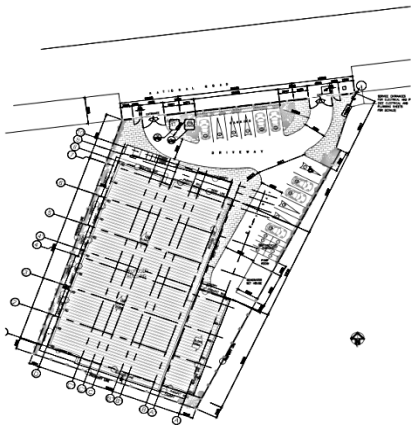
SITE DEVELOPMENT PLAN SCALE M-001
