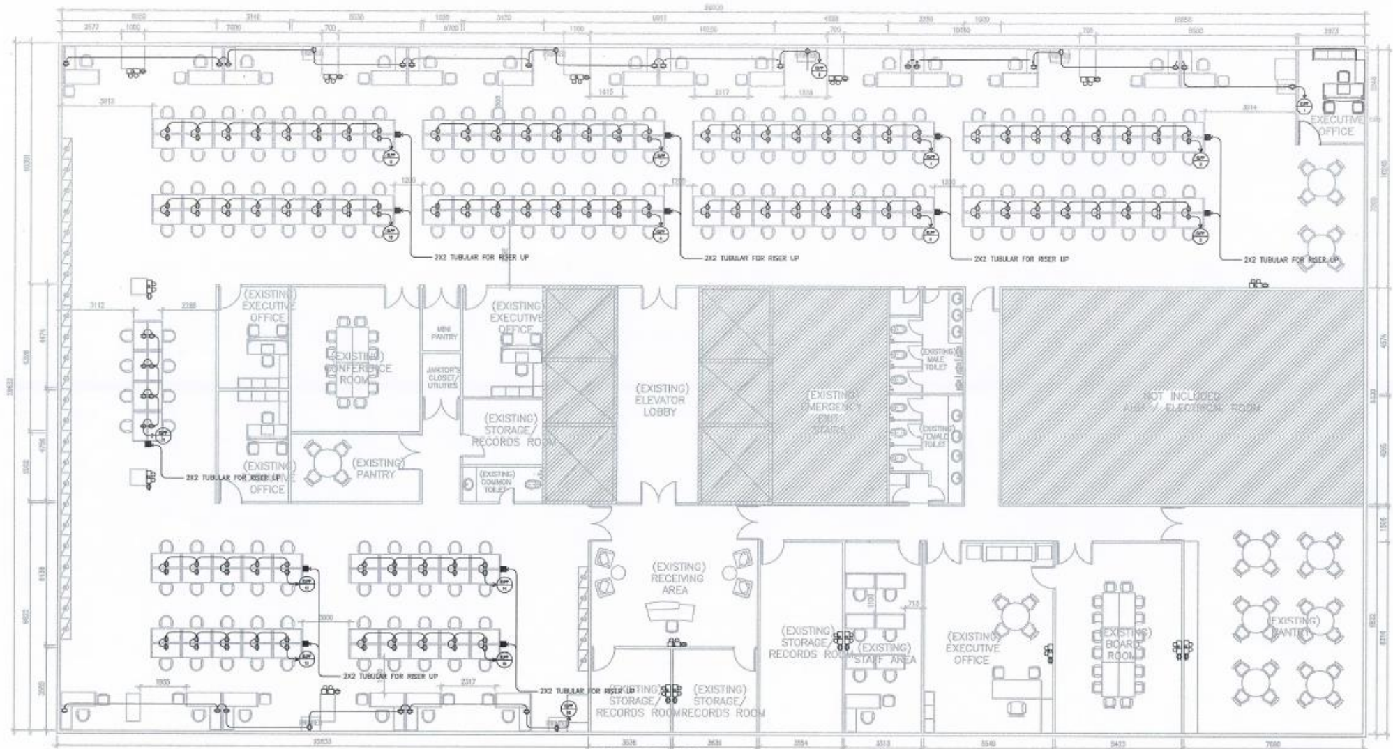
PROPOSED POWER LAYOUT 1 EE-06 SCALE : 1:150M
