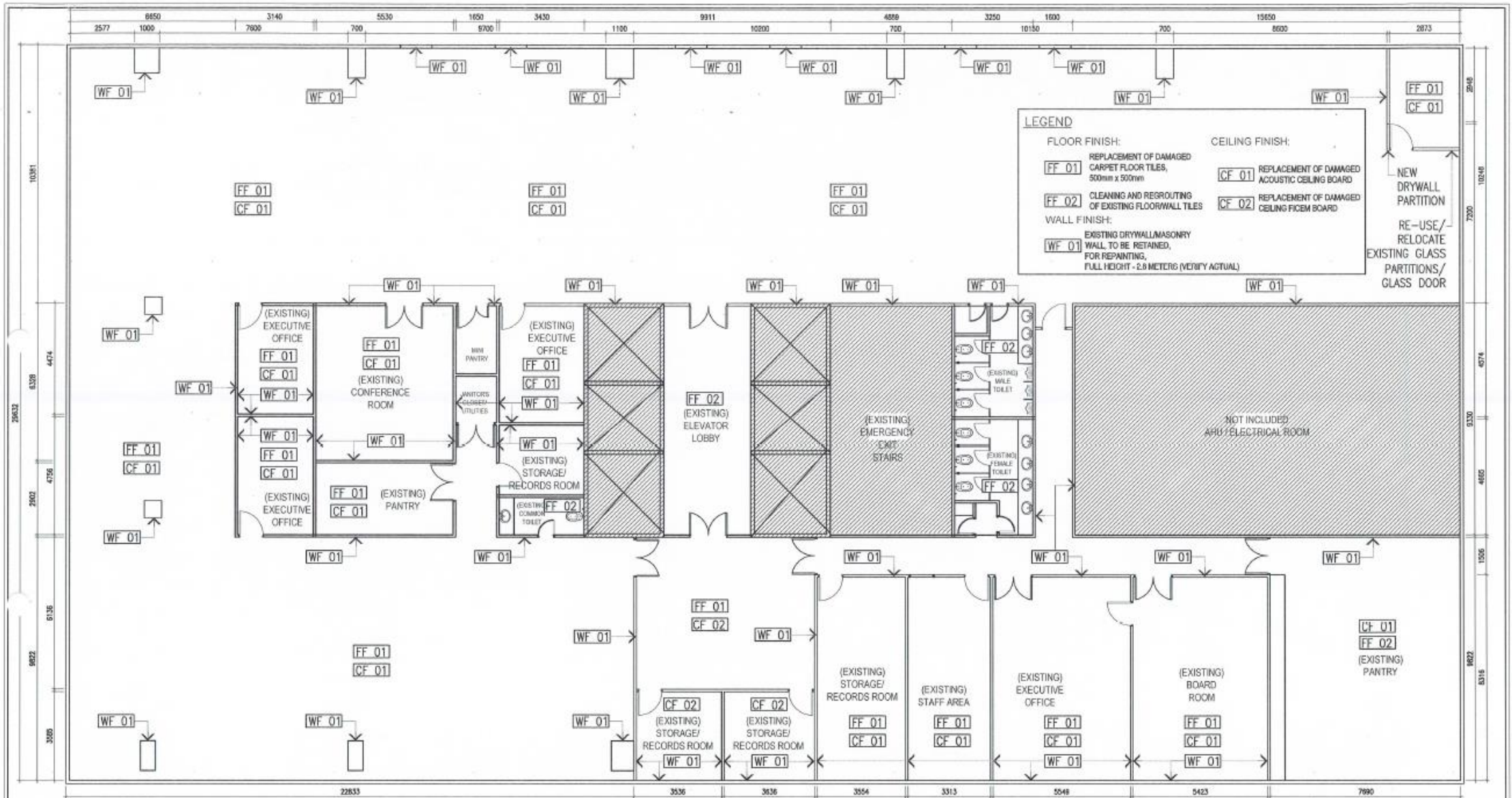
31st FLOOR - PROPOSED DESIGNATION PLAN 1 A-02 SCALE 1:100 M
